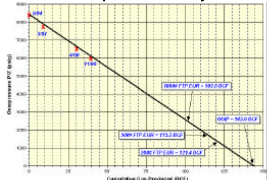
P/Z Overpressured Analysis
